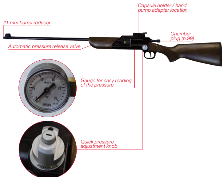
VERSATILE GAS PROJECTOR
